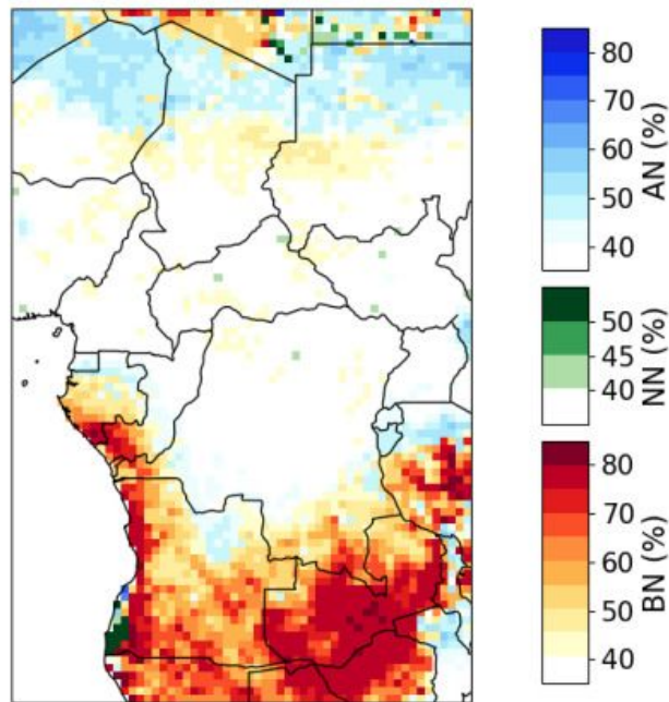
GEFSV12.PRCP - Probabilistic Forecast Week 2
