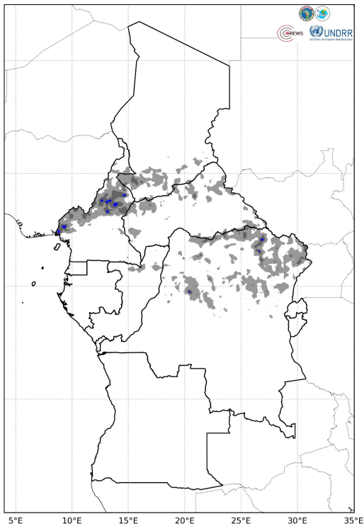
Weekly Observed Rainfall - IMERG (0.1°x0.1°) Period: 2026-06-29 to 2026-07-05
