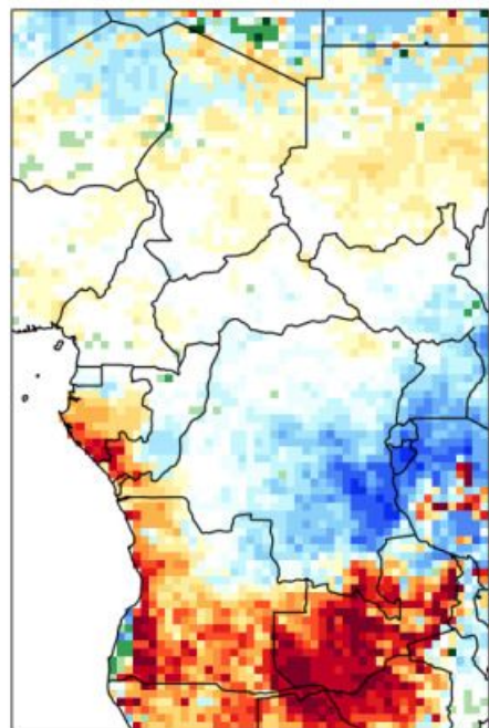
GEFSV12.PRCP - Probabilistic Forecast Week 4
