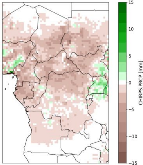
GEFSV12.PRCP - Deterministic Forecast Week 1
