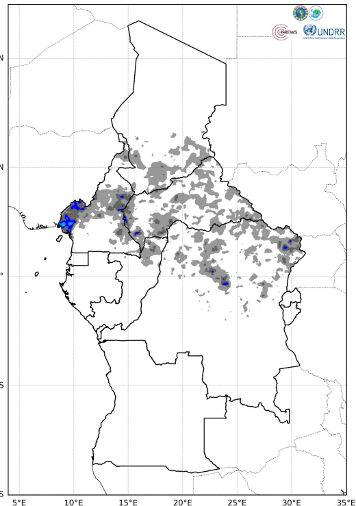
Weekly Observed Rainfall - IMERG (0.1°x0.1°) Period: 2026-07-06 to 2026-07-11
