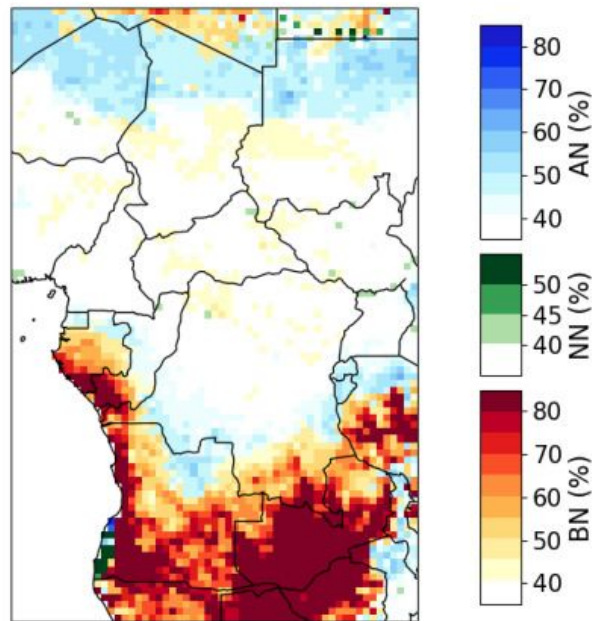
GEFSV12.PRCP - Probabilistic Forecast Week 1
