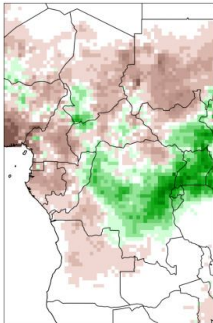
GEFSV12.PRCP - Deterministic Forecast Week 4
