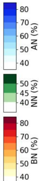
GEFSV12.PRCP - Probabilistic Forecast Week 4
