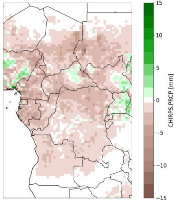
GEFSV12.PRCP - Deterministic Forecast Week 2
