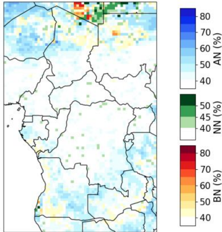
GEFSV12.PRCP - Probabilistic Forecast Week 3
