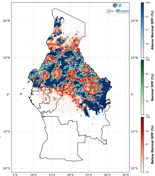
Standardized Precipitation Percentage (SPP) Valid Period: 2026-07-06 to 2026-07-11
