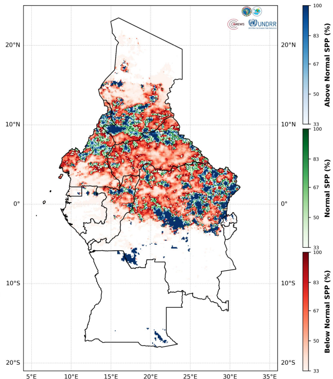
Standardized Precipitation Percentage (SPP) Valid Period: 2026-06-29 to 2026-07-05
