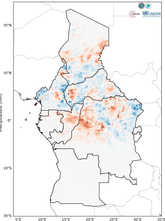
Observed IMERG Rainfall Anomaly Period: 2026-07-06 to 2026-07-11
