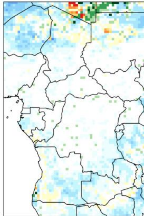
GEFSV12.PRCP - Probabilistic Forecast Week 3
