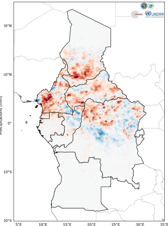
Observed IMERG Rainfall Anomaly Period: 2026-07-13 to 2026-07-18
