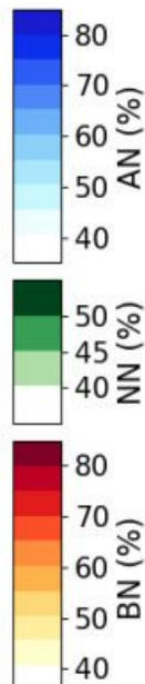
GEFSV12.PRCP - Probabilistic Forecast Week 4
