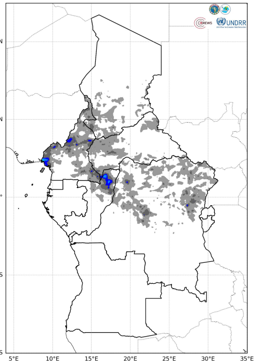
Weekly Observed Rainfall - IMERG (0.1°x0.1°) Period: 2026-07-13 to 2026-07-18
