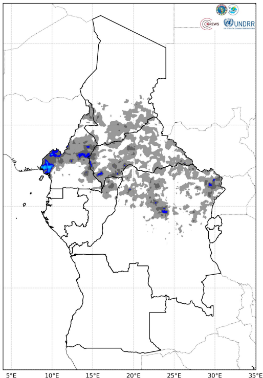
Weekly Observed Rainfall - IMERG (0.1°x0.1°) Period: 2026-07-06 to 2026-07-12
