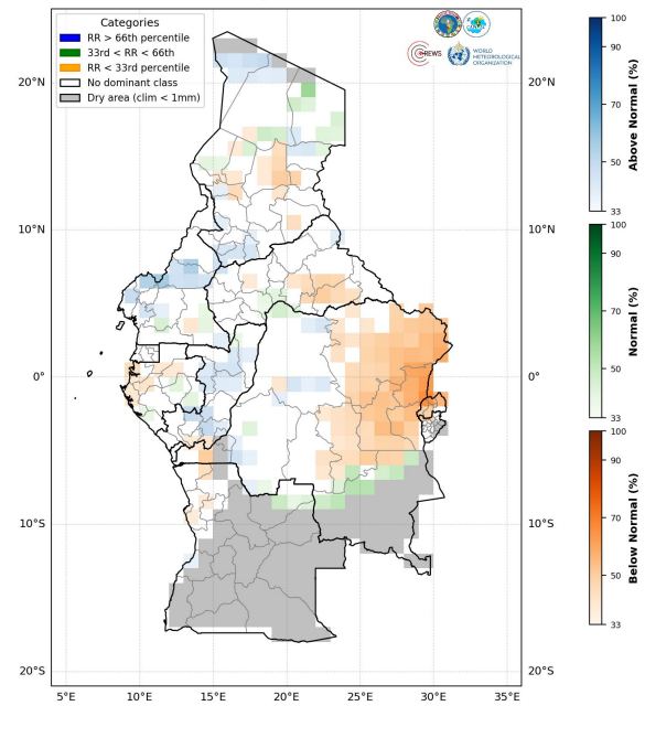
C3S Multi-Model Mean - Tercile Summary Semaine du 11 Aug au 17 Aug 2026 Init: June 2026
