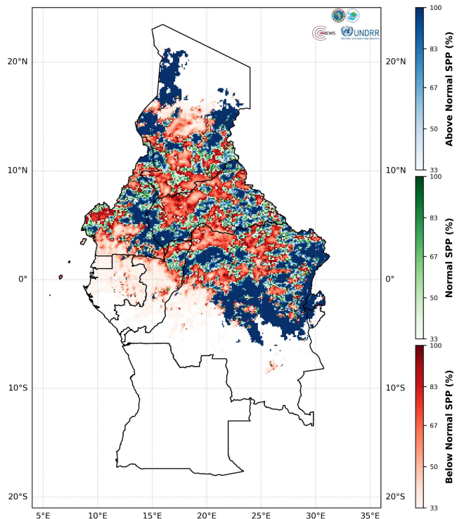
Standardized Precipitation Percentage (SPP) Valid Period: 2026-07-06 to 2026-07-12
