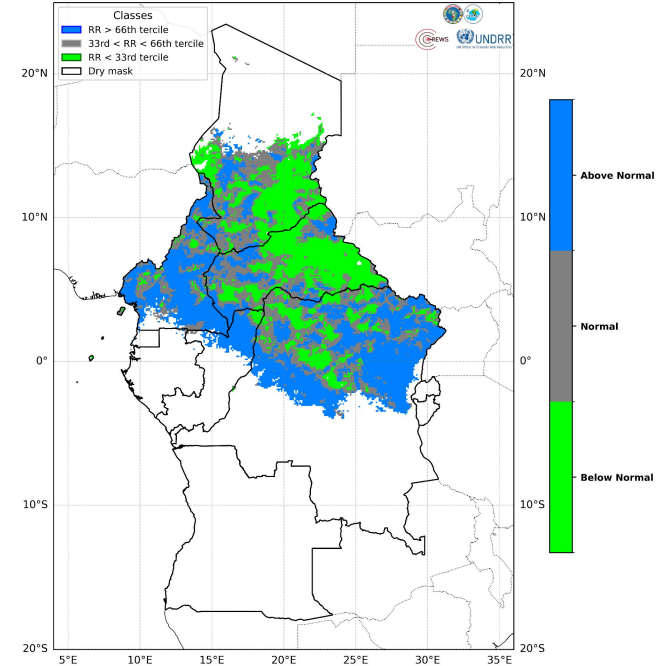
Observed Weekly Rainfall Categories (vs Climatology) Period: 2026-07-13 to 2026-07-18
