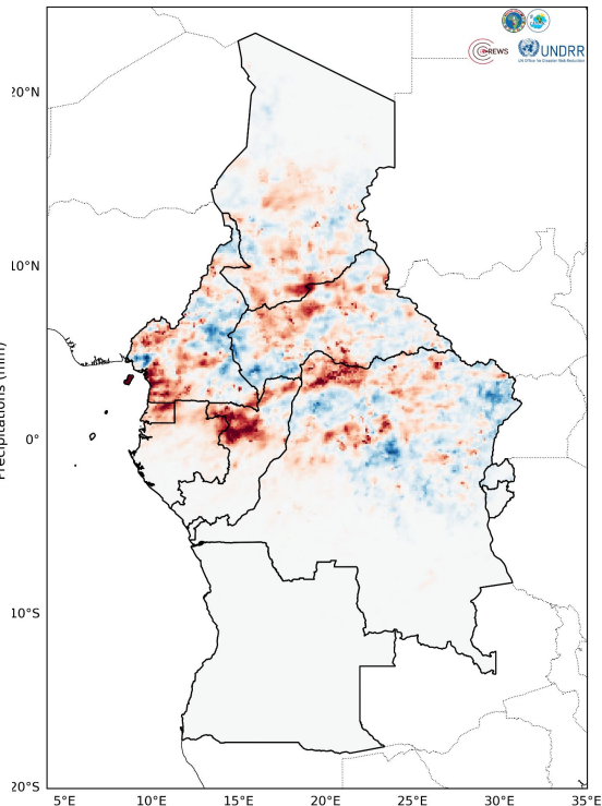
Observed IMERG Rainfall Anomaly Period: 2026-07-06 to 2026-07-12
