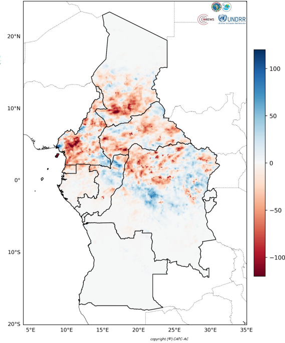
Observed IMERG Rainfall Anomaly Period: 2026-07-13 to 2026-07-18
