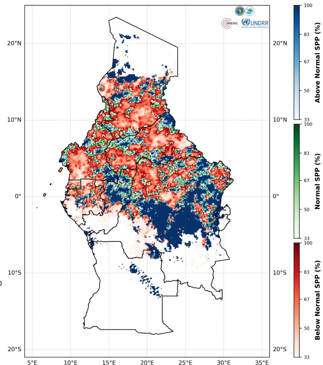
Standardized Precipitation Percentage (SPP) Valid Period: 2026-07-13 to 2026-07-18
