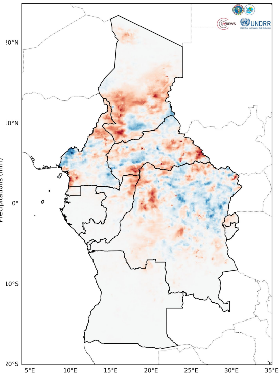
Observed IMERG Rainfall Anomaly Period: 2026-07-20 to 2026-07-26
