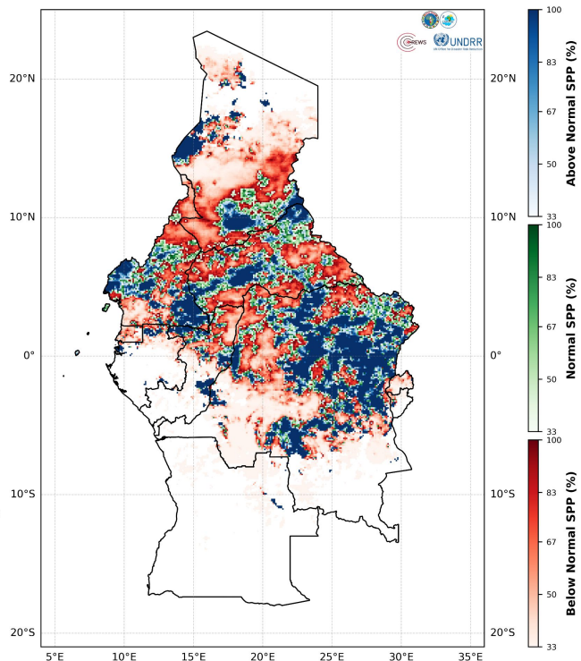
Standardized Precipitation Percentage (SPP) Valid Period: 2026-07-20 to 2026-07-26
