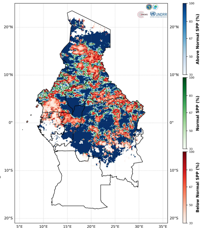
Standardized Precipitation Percentage (SPP) Valid Period: 2026-07-27 to 2026-08-01
