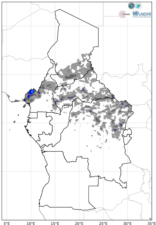
Weekly Observed Rainfall - IMERG (0.1°x0.1°) Period: 2026-07-20 to 2026-07-26
