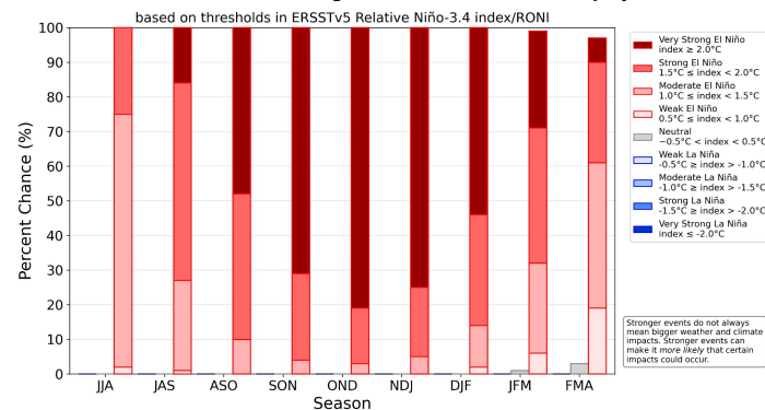
NOAA CPC ENSO Strength Probabilities (issued July 2026)
