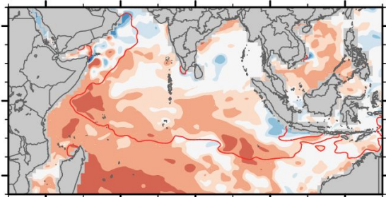
9-Aug to 15-Aug CFS Forecast
